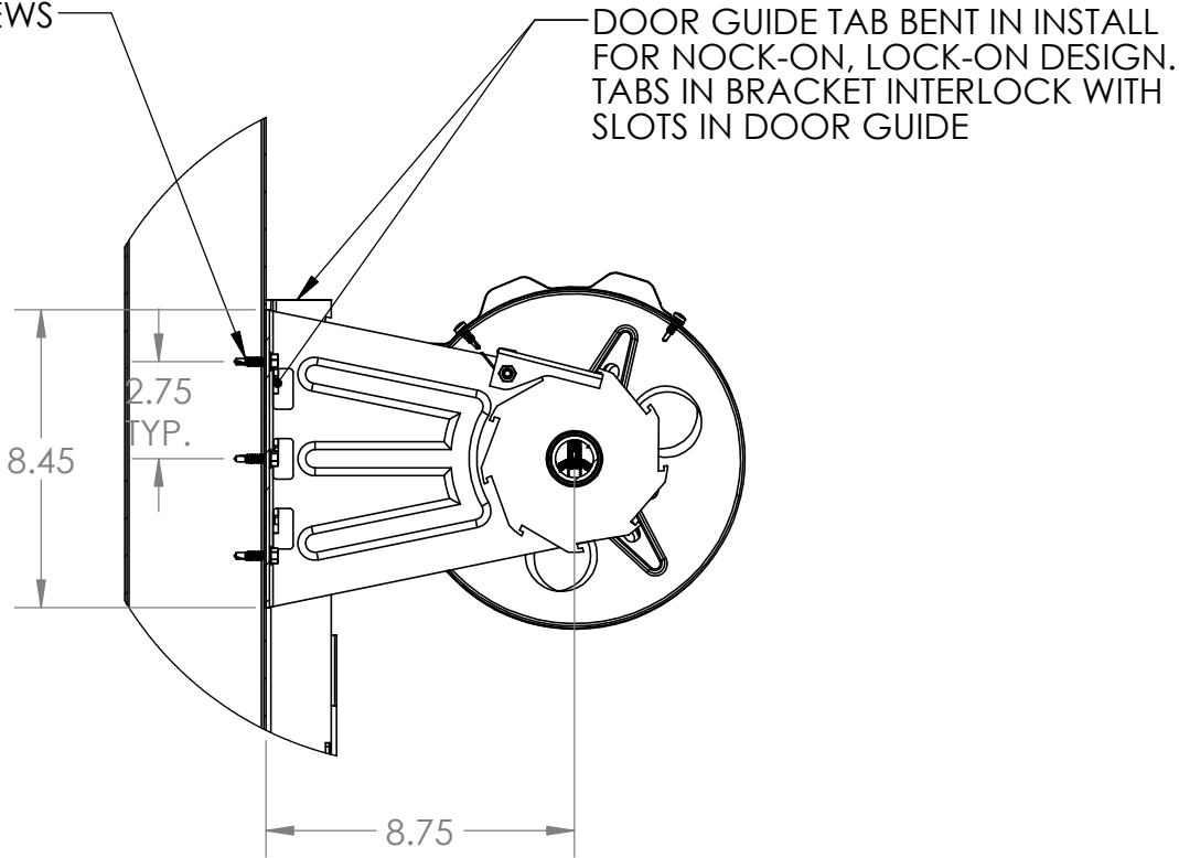
DOOR BRACKET TO STEEL JAMB
