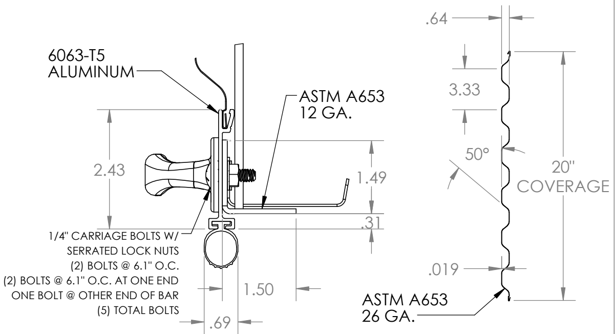
DOOR PANEL DETAIL
