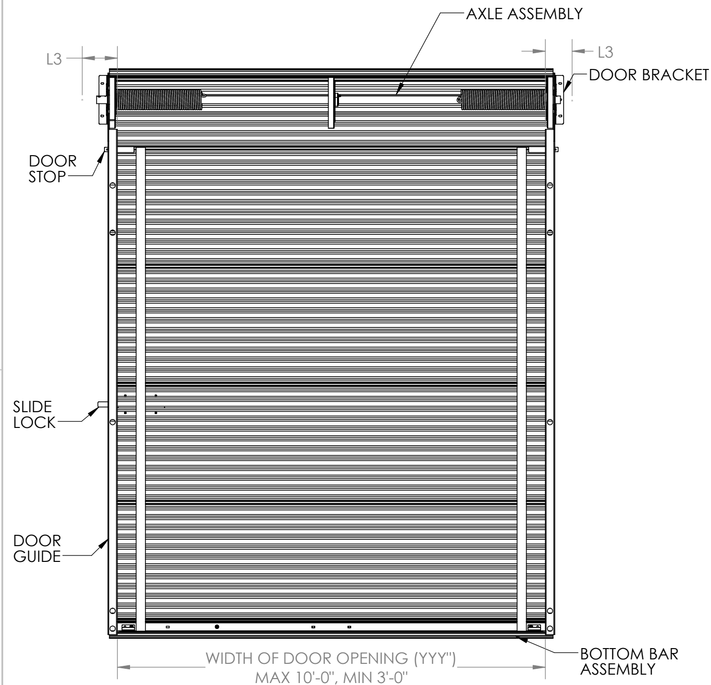
INSIDE ELEVATION
